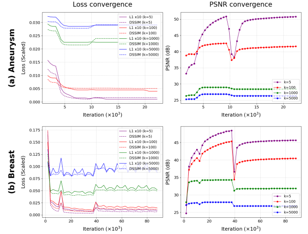
Fig. 7: Ablation on boundary sharpness ( k ) of differentiable ellipsoids on Aneurysm and Breast datasets.
