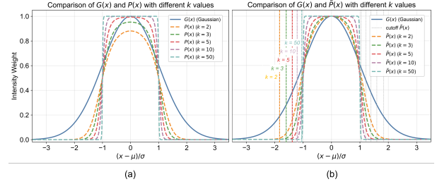
Fig. 1: 1D comparison between the Gaussian kernel G(x) and our sigmoid-based ellipsoid primitives with unit center intensity. (a) Effect of the sharpness parameter k on the primitive P(x) . Peak intensity decreases as k becomes smaller than 5. (b) Normalized primitive \tilde{P}(x) with corresponding cutoff regions for k = 2, 3, 5, 10, 50 .
