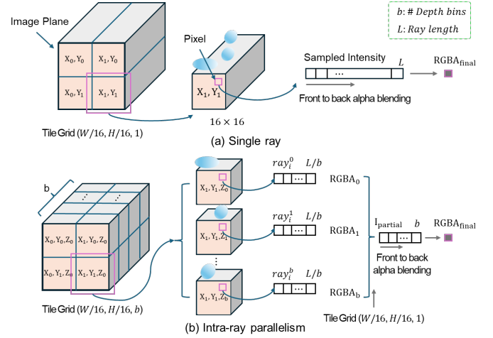
Fig. 7: Illustration of intra-ray parallelism.
