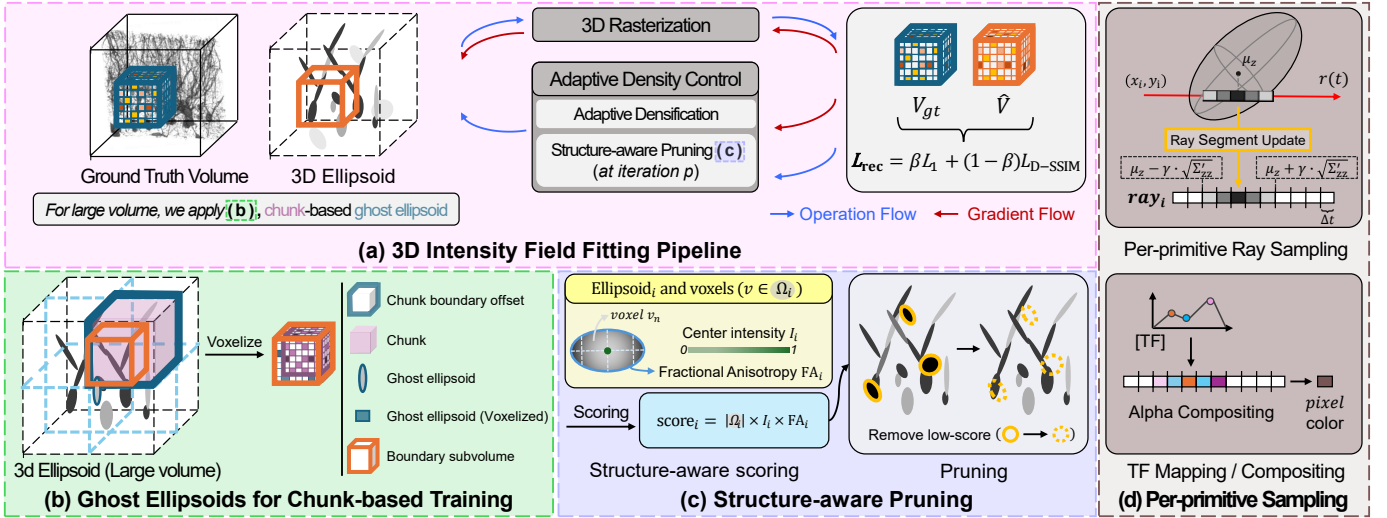
Fig. 3: Overview of our proposed framework: (a) 3D intensity field fitting pipeline, (b) chunk-based large volume training using ghost ellipsoid and (c) structure-aware pruning strategy, (d) per-primitive sampling and transfer function mapping of the intensity-fitted ellipsoids.
