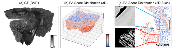
Fig. 9: Visualization of FA scores of ellipsoid primitives learned on a BigBrain chunk using our method. Red value indicates high FA score.
