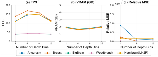
Fig. 8: Effect of depth bin count on (a) rendering performance (FPS), (b) GPU memory usage, and (c) rendering quality.
