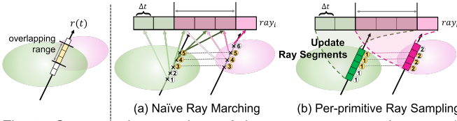
Fig. 6: Conceptual comparison of data access patterns between (a) naïve ray marching and (b) per-primitive ray sampling. In ray marching, primitive contributions are queried at each ray sample, causing repeated parameter loads. In contrast, our method processes each primitive once, determines its valid depth range, and updates only the affected ray segments, reducing redundant global memory traffic.
